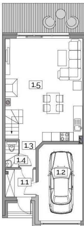
Parter 56,46 m 2
