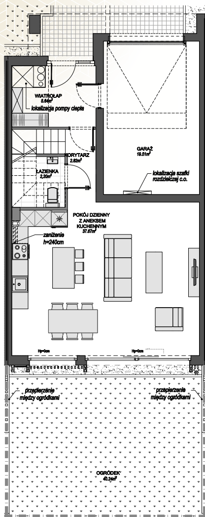
PARTER
