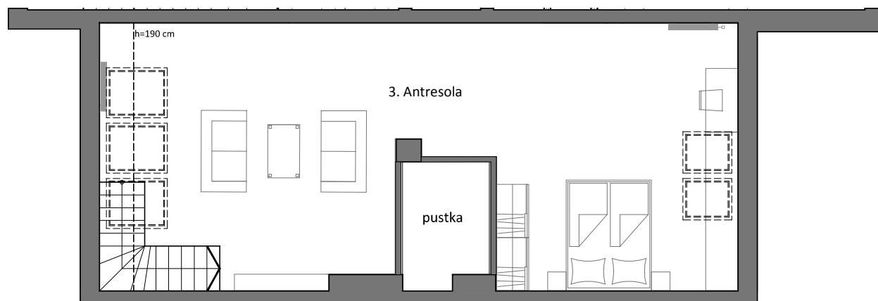
ANTRESOLA
