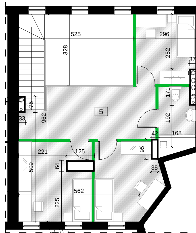
RZUT M14 ANTRESOLI
