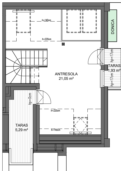
ANTRESOLA
